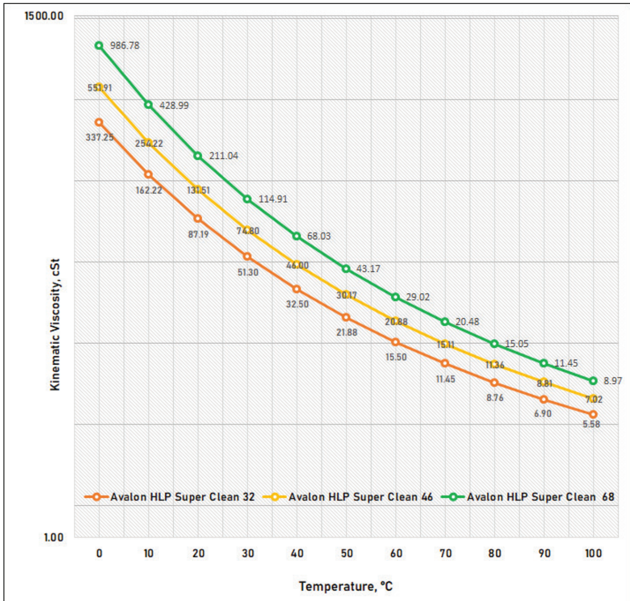
Diagram for Avalon HLP Super Clean
